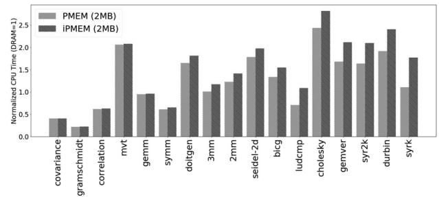
Fig. 3. Polybench: Cases where PMEM (non-interleaved PMEM) faster than iPMEM (interleaved PMEM) — interleaving does not provide substantial benefit in these cases; surprising because we expect the 2 MB page size to dominate.
