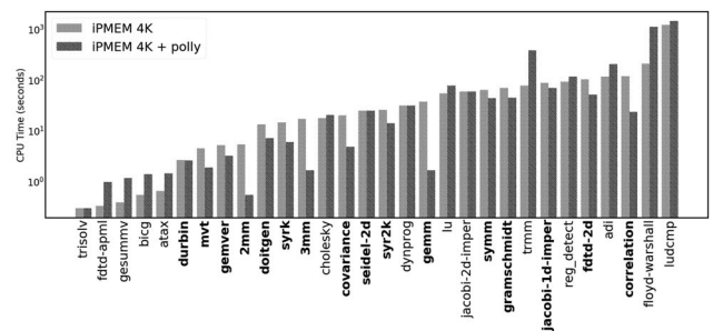
Fig. 4. Polyhedral Memory optimizations for interleaved PMEM (iPMEM), 4K and 2M pages. Varying cache layers impact performance differently. Results sorted by execution time without polyhedral optimization. Boldface indicates improvement with poly optimization.
