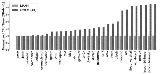
Fig. 2. Polybench: DRAM versus Interleaved PMEM (both 4K pages). Results closer to expectations but still better than expected. Caching masks lower bandwidth of PMEM; memory usage optimization improves cache benefits which improves performance and decreases benefit of PMEM interleaving. Sorted by PMEM performance.
